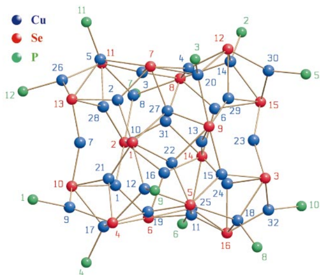
Fig. 1 Molecular structure of [\text{Cu}_{32}\text{Se}_{16}(\text{PPh}_3)_{12}] 2 . \text{Cu}^{+} : blue; \text{Se}^{2-} : red; P: green. Cu–Cu contacts and carbon atoms are omitted for clarity. Cu, Se and P atoms are labelled with blue, red and green numbers respectively.
