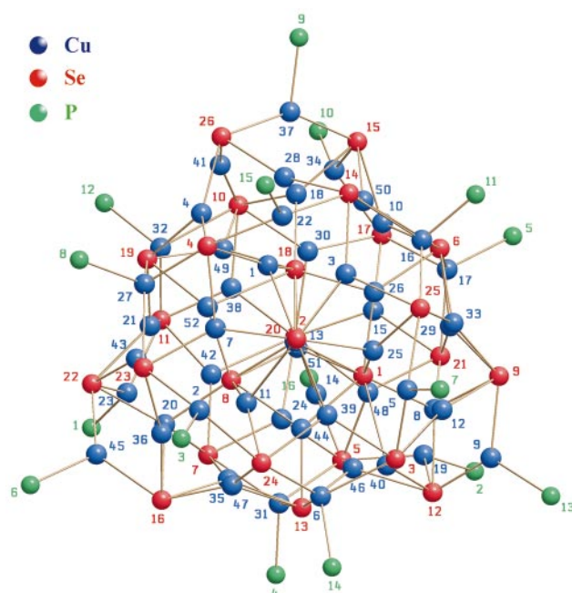
Fig. 2 Molecular structure of [\text{Cu}_{52}\text{Se}_{26}(\text{PPh}_3)_{16}] 3 . \text{Cu}^{+} : blue; \text{Se}^{2-} : red; P: green. Cu–Cu contacts and carbon atoms are omitted for clarity. Cu, Se and P atoms are labelled with blue, red and green numbers respectively.
